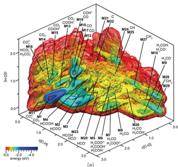
Fig. 10 Free energy landscape from the metadynamics sampling of methanol synthesis based on CO 2 over the reduced Cu 8 /ZnO(000 \bar{1} ) catalyst surface model (a). The coordination numbers c[C–O], c[C–H], and c[O–H] (see text) were employed as collective variables (CVs) to describe the interaction of the carbon atom with the oxygen atoms of the top layer of ZnO and the two oxygen atoms of the reactant CO 2 , the carbon atom with all hydrogen atoms in the system, and all hydrogen atoms with the two oxygen atoms of the reactant CO 2 , respectively. Relative free energies \Delta F are reported according to the shown color scale. Bold capital M plus a number labels distinct free energy minima. Reprinted with permission from ref. 222. Copyright 2015 American Chemical Society.
