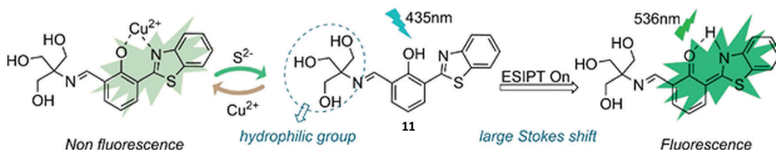
Scheme 12 Development of a reversible ESIPT fluorescent probe 11 for the detection of copper or S^{2-} . Measurement conditions: PBS solution (10 mM, pH 7.4). Reproduced with permission from ( Sens. Actuators, B , 2018, 256 , 600–608). Copyright (2018) Elsevier.
