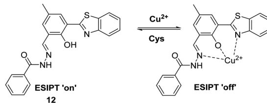
Scheme 13 An ESIPT-based fluorescent probe 12 for the reversible detection of Cu 2+ and Cys. Measurement conditions: PBS/ACN (8 : 2), pH 7.4.
