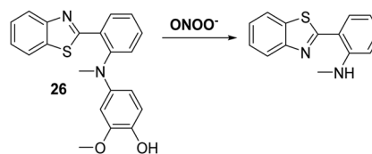
Scheme 24 A reaction-based fluorescent probe 26 that allows for the rapid detection of ONOO − in cells and within a live mouse brain. Measurement conditions: PBS solution (10 mM, pH = 7.4).
