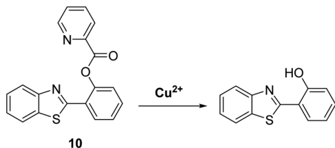
Scheme 11 Selective hydrolysis of picolinoyl ester of probe 10 and its use for the fluorescence detection of Cu 2+ . Measurement conditions: PBS/ACN (8:2) – pH 7.4.
