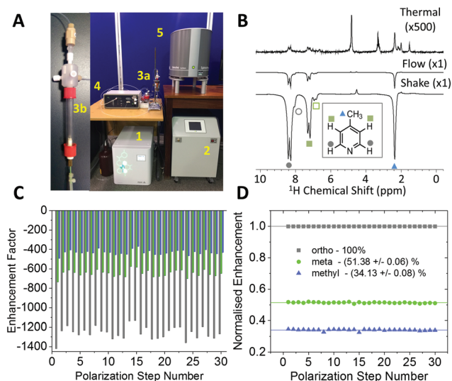
Fig. 5 (A) Automated SABRE flow system that includes: (1) electrolysis cell, (2) Bruker p\text{-H}_2 conversion unit, (3a) PTF solenoid coil, (3b) mixing chamber, (4) Bruker polarizer control unit, and (5) 43 MHz (1 T) Magritek Spinsolve Carbon NMR spectrometer. (B) ^1\text{H} NMR spectra of 52 mM 4-methylpyridine with 5.2 mM catalyst in methanol- d_4 acquired with (top) thermal polarization, (middle) SABRE hyperpolarization using the automated flow system, (bottom) SABRE hyperpolarization using manual shaking. Both SABRE spectra were acquired with a PTF \sim 63 G. (C) Variability between repeated SABRE hyperpolarization experiments where the sample is repolarized between each acquisition. (D) Data from (A) normalized to the enhancement factor of the ortho resonance.
