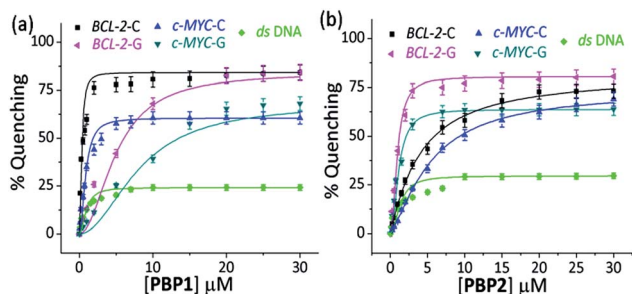
Fig. 2 The percentage fluorescence quenching observed upon titration of 250 nM of 5'-TAMRA labeled folded BCL -2-C and c -MYC-C i-motif structures in 60 mM K-cacodylate buffer, pH 6, and 250 nM 5'-TAMRA labeled folded BCL -2-G and c -MYC-G G-quadruplex structures in 60 mM K-cacodylate buffer, pH 7 by (a) 0–30 \mu M PBP1 and (b) 0–30 \mu M PBP2 .
