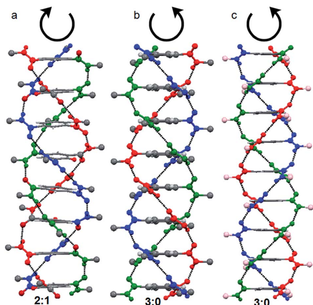
Fig. 1 (a) M helix from a trisamide with 2 : 1 conformations containing achiral \beta -alanine. (b) P helix by a trisamide with 3 : 0 conformations containing achiral \gamma -aminobutyric acid. (c) The trisamide containing chiral methionine (pink balls) adopts 3 : 0 conformations and formed P helix. Amino acids side chains are omitted for clarity.
