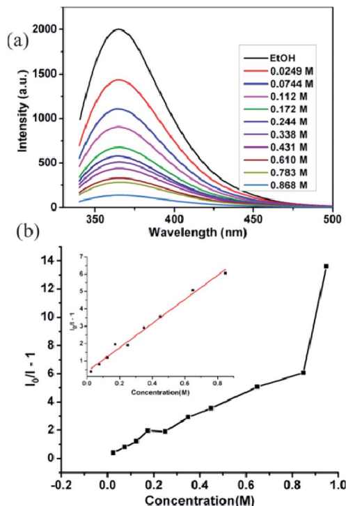
Fig. 7 (a) Fluorescence titration dispersed in ethanol by gradual addition of acetone, (b) The curve of (I_0/I - 1) vs. acetone concentration in compound 2. Inset is the linear plot at low concentration.
