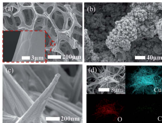
Fig. 7 Field emission SEM (FE-SEM) images of (a) PGF, (b) \text{Cu}(\text{OH})_2/\text{PGF} and (c) \text{Cu}(\text{OH})_2 single nanorod; (d) FE-SEM image of \text{Cu}(\text{OH})_2/\text{PGF} and energy dispersive spectroscopy (EDS) elemental mappings of copper, oxygen, and carbon atoms (reproduced with permission from Elsevier: Shackery et al. 2016).
