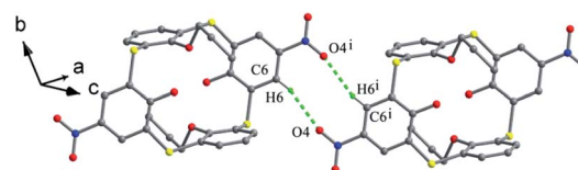
Fig. 90 A dimer of 101 , showing C–H \cdots O H-bonds.
