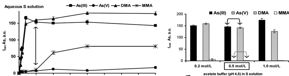
Fig. 2 Effect of acidity related to the \text{CH}_3\text{COOH} concentration in the S and A solutions on the measurements of As(III), As(V), DMA and MMA ( 20 \text{ ng g}^{-1} each) by HG-ICP OES using the 1.0% \text{NaBH}_4 R solution. Left side: \text{CH}_3\text{COOH} was used for the HG reaction. Simple S solutions (not acidified with HCl) and the A solution containing \text{CH}_3\text{COOH} at various concentrations were used. Right side: acetate buffer at adjusted pH was used for the HG reaction. The S solutions were acidified with the acetate buffer (pH 4.5), the use of the A solution was excluded.
