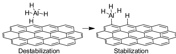
Scheme 16 Proposal for the mechanism of NaAlH 4 decomposition by activation at the edges of G.
