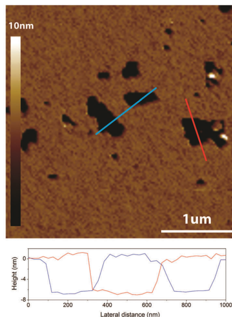
Fig. 5 Left panel: The percentage of friction experiments performed at a given temperature where the load bearing capacity was found to be less than 20 nN. The number shown in each column is the total number of experiments performed at a given temperature. Right panel: AFM topographical image of a DPPC bilayer with defects in PBS buffer solution. Height lines over the regions marked with the corresponding colors on the topographical image are shown below the image. The temperature was 32 °C. Reproduced with permission from ref. 37 © 2017 Elsevier Inc.
