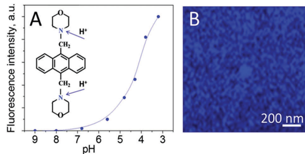
Fig. 3 (A) Calibration of fluorescent pH indicator, 4,4'-(anthracene-9,10-diylbis(dimethanedimethylammonium))diphenylmethane, that exhibits a pK_a \sim 5.1 , and initial chemical formula showing the protonation sites; (B) confocal fluorescent images of the TiO_2 surface immediately after irradiation.
