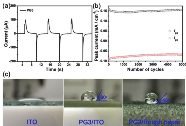
Fig. 4 (a) Chronoamperometry for PG3 with a 5 s delay for each potential ( -0.1 V and +0.8 V). (b) Stability of a 600 nm thick PG3 film cycled 5000 times with a scan rate of 100 mV s^{-1} in 0.1 M TBAPF 6 /ACN: the change in the anodic ( \square ) and cathodic ( \circ ) peak currents as a function of number of cycles. (c) Photographs of the water droplet volume of 10 \mu L on the surface of ITO, PG3/ITO and PG3/rough paper, respectively.
