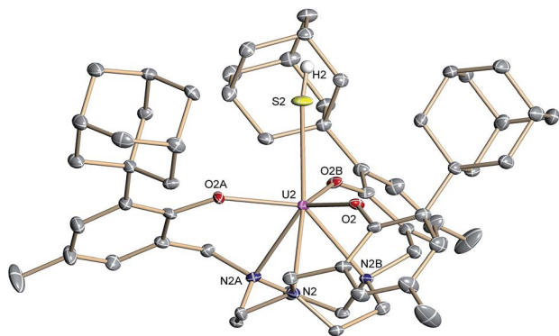
Fig. 1 Molecular structure of the uranium(IV) hydrosulfido complex [[(\text{Ad}, \text{MeArO})_3\text{tacn}]\text{U}-\text{SH}] ( 2 ) with the chalcogen-bound H atom located in the difference Fourier map. All other hydrogen atoms and the solvent molecules are omitted for clarity (50% probability ellipsoids).
