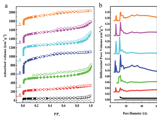
Fig. 2 (a) Nitrogen gas adsorption isotherms measured at 77\text{ K} and STP, and (b) the curves of the pore size distributions calculated via the NLDFT method for \text{C}_{60} (gray), PAF-60-a (black), PAF-60-b (red), PAF-60-c (green), PAF-60 (blue), PAF-60-e (cyan), PAF-61 (purple), and PAF-62 (orange) from the bottom to the top.
