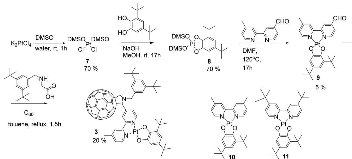
Scheme 2 Alternative synthetic route towards the donor-acceptor complex 3 via the Prato reaction of the aldehyde group tagged bipyridine-Pt-catecholate unit and C 60 fullerene. Molecular structures of the model dyads (4,4'-diMe-bpy)Pt(cat) ( 10 ) and (4,4'-di t Bu-bpy)Pt(cat) ( 11 ) are also shown.
