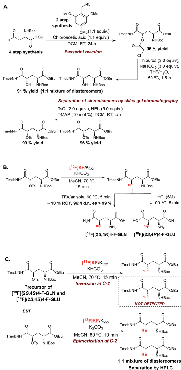
Scheme 2 (A.) Synthesis of the substrates for the radiosynthesis of [^{18}\text{F}] 4-F-GLU and [^{18}\text{F}] 4-F-GLN. (B.) Radiosynthesis of [^{18}\text{F}](2\text{S},4\text{R}) 4-F-GLU and [^{18}\text{F}](2\text{S},4\text{R}) 4-F-GLN. (C.) Radiosynthesis of [^{18}\text{F}](2\text{S},4\text{S}) 4-F-GLU and [^{18}\text{F}](2\text{S},4\text{S}) 4-F-GLN precursors. Tmob = 2,4,6-trimethoxybenzyl.
