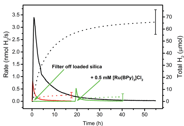
Fig. 2 Hydrogen evolution rate courses (solid lines) and total amounts of H 2 (dotted lines) in 1 M ascorbate buffer (pH 4) with 0.1 M NaOTf. Black: 20 μM 3 and 200 μM 5 adsorbed on hydrophobic fumed silica with 300 μM [C 16 -NMe 3 ][OAc] ( 7 ) as surfactant. Green: same as black, but loaded silica was filtered off and the residual solution irradiated, then 0.5 mM [Ru(bpy) 3 ]Cl 2 was added and irradiation continued (green arrows). Red: 0.5 mM [Ru(bpy) 3 ]Cl 2 , no WRC. See Table S13.†
