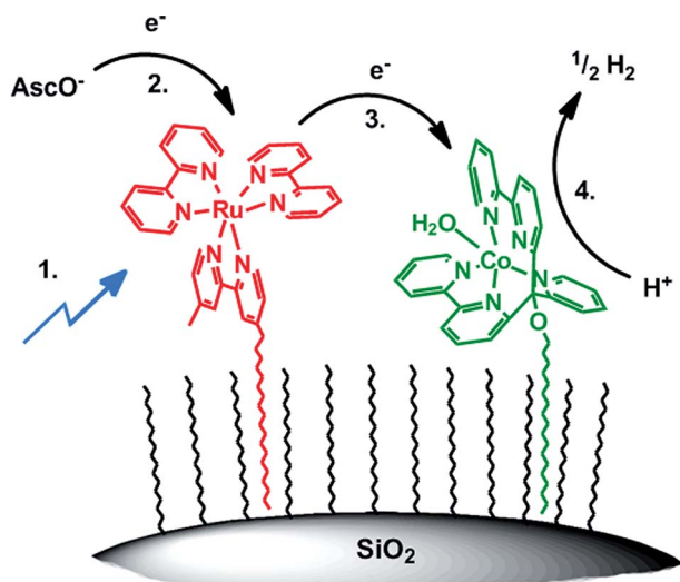
Scheme 4 Proposed reaction mechanism of photocatalytic \text{H}_2 production on hydrophobic silica: (1) photoexcitation of 5 \rightarrow 5* ; (2) reductive quenching of 5* \rightarrow 5 - ; (3) electron transfer 5 - \rightarrow 3 ; (4) \text{H}^+ reduction by 3 - .
