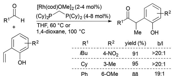
Scheme 1 Hydroacylation of vinylphenols with non-chelating aldehydes.
