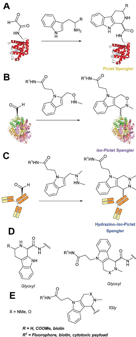
Scheme 10 (A) The Pictet-Spengler ligation on glyoxyl-myoglobin. (B) The iso-Pictet-Spengler ligation on fGly-tagged maltose binding protein. (C). The Hydraizo-iso-Pictet Spengler ligation on an fGly-tagged antibody. (D). The Pictet Spengler (left) and iso-Pictet/Hydraizo-iso-Pictet Spengler ligation at a glyoxyl handle. (E). The iso-Pictet Spengler/Hydraizo-iso-Pictet Spengler ligation at an fGly handle.
