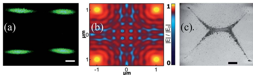
Fig. 4 Plasmo-fluidic assembly of nanoparticles using quadruple-trap configuration. (a) Optical dark-field image of the four, evanescently-excited 532 nm laser spots on a gold film (50 nm thick) optically coupled to the Dove prism. Scale bar is 200 \mu\text{m} . (b) Simulated electric near-field distribution of the four laser spots at the gold–water interface. The geometry of the simulation was identical to the experimental configuration. Plasmonic interference patterns can be clearly observed. (c) Optical bright-field image of plasmo-fluidic assembly of Ag nanoparticles at gold film–water interface due to excitation shown in (a). Scale bar is 200 \mu\text{m} . The nanoparticle densities at the corners of the geometry are different due to small variance in the laser powers.
