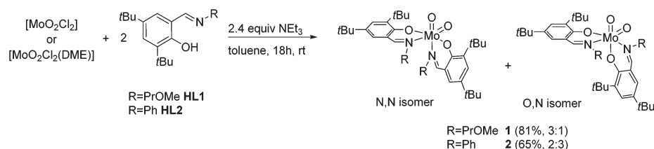
Scheme 2 Synthesis of molybdenum(VI) dioxido complexes 1 and 2 and their respective isomeric ratios (N,N : O,N).
