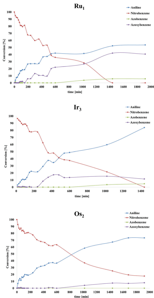
Fig. 1 Time-dependence screening for the selected complexes Ru 1 , Ir 3 and Os 2 .
