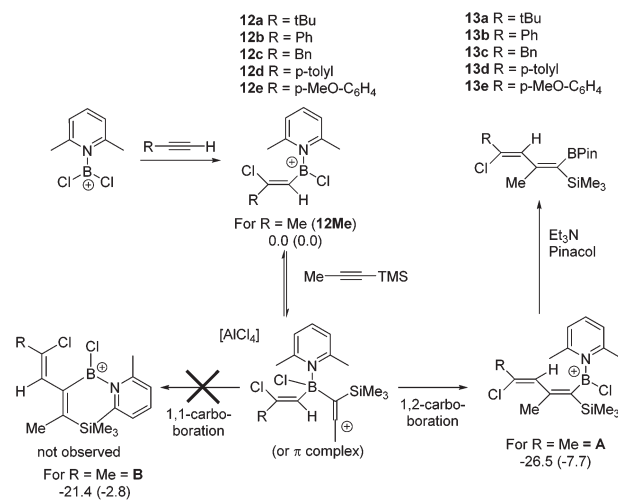
Scheme 4 1-Boradiene formation by haloboration and 1,2-carboboration. Electronic energies (Gibbs free energies at 293 \text{ K} ) shown in \text{kcal mol}^{-1} for the model system where \text{R} = \text{Me} (all energies relative to 12Me and 1-TMS-1-propyne at infinite distance).
