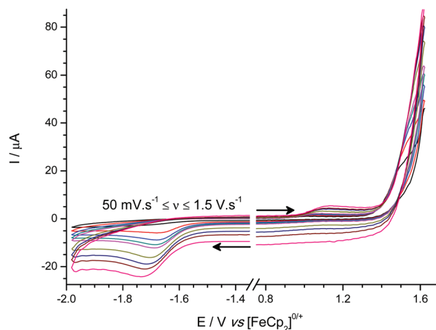
Fig. 6 Experimental cyclic voltammogram(s) for the oxidation of [tmpH][(μ-H)(1) 2 ].
