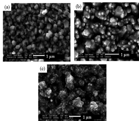
Fig. 4 SEM images of CdS thin films deposited from [\text{Cd}(\text{S}_2\text{CNC}_5\text{H}_{10})_2\text{-py}] at (a) 350 °C; (b) 400 °C and (c) 450 °C. Reproduced from ref. 40 with permission from the Centre National de la Recherche Scientifique (CNRS) and the Royal Society of Chemistry.
