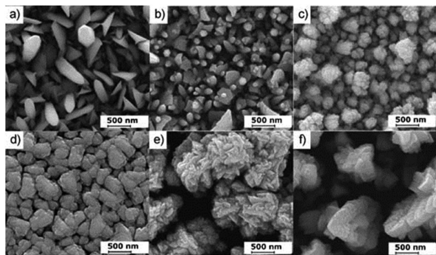
Fig. 3 SEM images of CdS thin films deposited from [Cd(S 2 CNCy 2 ) 2 ·py] on FTO (a–c) and soda glass (d–f) at 350, 400, and 450 °C from THF solution. Reproduced with permission from ref. 37. Copyright 2012 Wiley.
