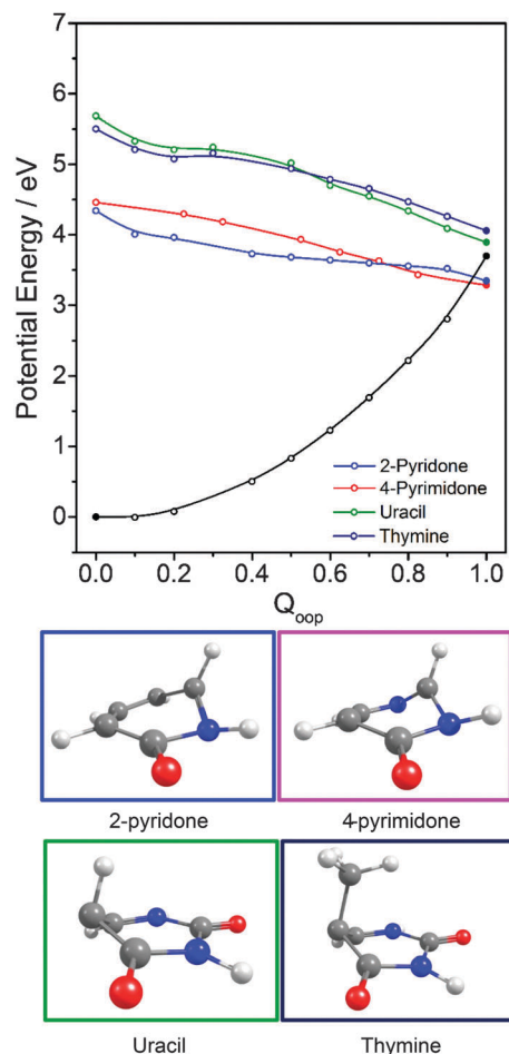
Fig. 11 Overlaid PECs along Q_{\text{oop}} for the 1^1\pi\pi^*/S_0 MECI states and respective 1^1\pi\pi^*/S_0 MECIs for 2-pyridone, 4-pyrimidone, U and T along with the calculated S_0 PEC for 2-pyridone. The filled points show the energies of the optimised critical structures ( i.e. the S_0 state and the S_0/1^1\pi\pi^* CI). The optimised geometry at each MECI is shown below.
