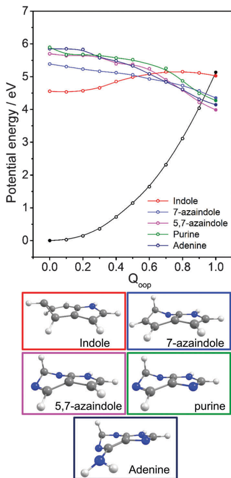
Fig. 13 Overlaid diabatic PECs along Q_{oop} for the 1^1\pi\pi^*/S_0 MECI in indole, 7-azaindole, 5,7-azaindole, purine and A. The filled points show the energies of the optimised critical structures (i.e. the S_0 state minimum and the S_0/1^1\pi\pi^* MECI) and, for clarity, only the S_0 PEC calculated for indole is shown (open black points). The optimised geometry at each MECI is shown below.
