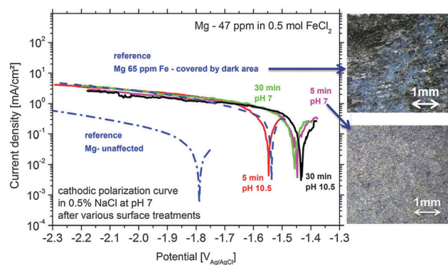
Fig. 3 Increased cathodic activity of Mg-47 ppm Fe samples after immersion treatments in 0.5 M \text{FeCl}_2 solution for 5 and 30 min at pH 7 and 10.5. For comparison the initial bare- and corroded Mg-65 ppm Fe with the fully corroded surface are shown. The dark surface appearance of two test samples is shown by optical micrographs (initially all had a shiny surface).
