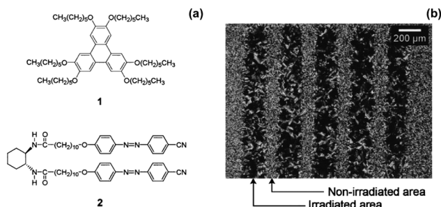
Fig. 5 (a) Molecular structures of 1 and 2 (b) optical polarized light microscope image of a patterned sample of 1 , 2 at 65 °C prepared by cooling under UV light using a photomask. Adapted from ref. 73 with permission from the Royal Society of Chemistry.
