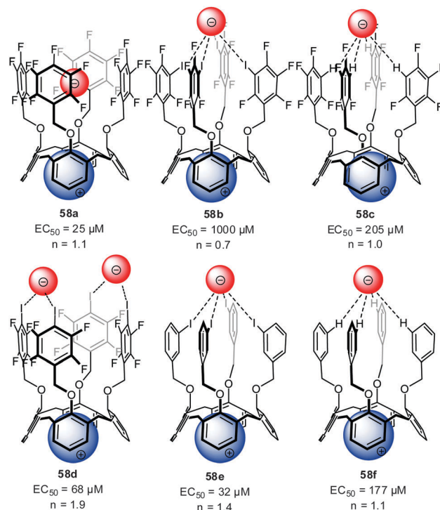
Fig. 32 Molecular structure of the investigated ion pair receptors 58 for transport studies by Metrangelo, Resnati and Matile et al. 10a
