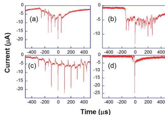
Fig. 8 Chronoamperometric current obtained for the reduction of K_3[Fe(CN)_6] (50 mM) in aqueous KNO_3 under ultrasound power of 8.9\text{ W cm}^{-2} at a 29\text{ }\mu\text{m} diameter platinum electrode. Horn-to-electrode distances are 10 mm (a–c) and 1 cm (d). Adapted from ref. 67.
