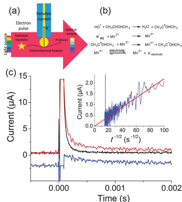
Fig. 12 (a) Principle of electrochemical detection of intermediates created by pulse radiolysis. (b) Chemical reactions leading to production of MV^{\bullet+} . (c) Transient electrochemical signal observed when a solution containing 1 mM MV^{2+} , 0.35 M Na_2SO_4 and 50 mM isopropanol was irradiated with a pulse of 25 Gy. Black: parasitic signal obtained when the electrode is placed outside the beam. Red: electrochemical signal obtained when the electrode is positioned on the electron trajectory. Blue: faradaic signal obtained by subtraction ( -2 \mu A offset was applied for clarity) Inset: I versus t^{-1/2} and linear fit of the faradaic signal. Adapted from ref. 88.
