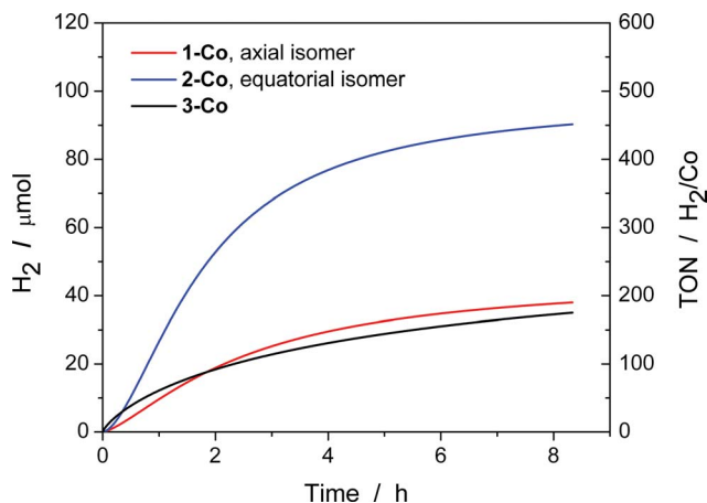
Fig. 8 Photocatalytic H_2 production of 1-Co, 2-Co, and 3-Co with [Ru(bpy)_3]^{2+} and ascorbic acid under 452 \pm 10 nm (540 mW). H_2 evolution and TON vs. time measured over 8 h of photocatalysis. Conditions: 2.0 \times 10^{-5} M Co(II) catalyst, 3.3 \times 10^{-4} M [Ru(bpy)_3]^{2+} , and 0.3 M H_2A/HA^- at pH 5.5.
