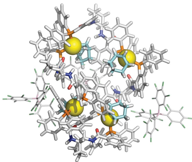
Fig. 6 MM3 structure of tetranuclear cyclo-oligomer ([\mathbf{1}][\text{BAR}_F])_4 . For clarity, only two of the four BAR F anions are shown. Colour coding: Pd, yellow; P, orange; O, red; N, dark blue; C, light grey; B, pink; F, green; \eta^3\text{-C}_6\text{H}_9 , light blue.
