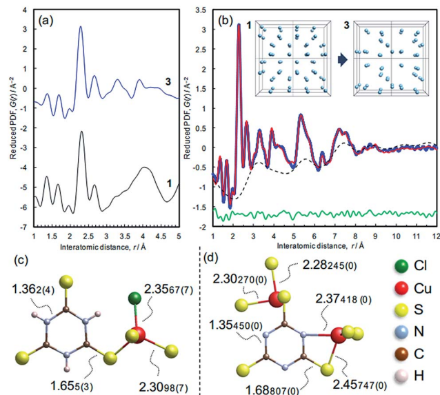
Fig. 6 X-ray pair distribution function analysis. (a) Experimental PDF pattern of 3 and simulated pattern of 1 . (b) PDF refinement of the structure of 3 . The model consists of (i) the \text{ttc}^{3-} anions coordinating to two Cu atoms as shown in panel d, which generate the sharp peaks, and (ii) the arrangement in space of these units, which generates the broad oscillating background (dotted line). The latter was simulated by moving the coordinates of the Cu sites in 1 to fit the broad oscillation as illustrated in the inset. (c) Local structure and bond lengths of 1 , determined by single crystal X-ray diffraction. (d) Representative local structure and bond lengths in 3 , determined by the PDF refinement.
