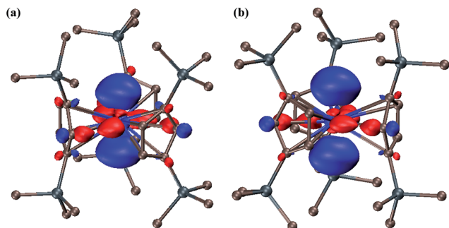
Fig. 3 Contour plots of (a) the LUMO of \text{Cp}_3^*\text{Th} and (b) the HOMO of the (\text{Cp}_3^*\text{Th})^{1-} anion in 3. Contour value is 0.05.
