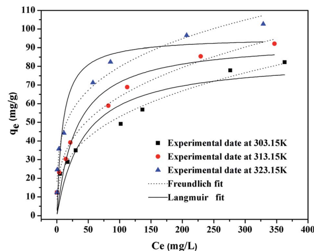
Fig. 10 Freundlich and Langmuir isotherms of Cr(vi) adsorption on zinc-biochar (Cr(vi) solution volume: 50 mL; adsorbent dose: 0.1 g; contact time: 24 h; pH: 2.0).
