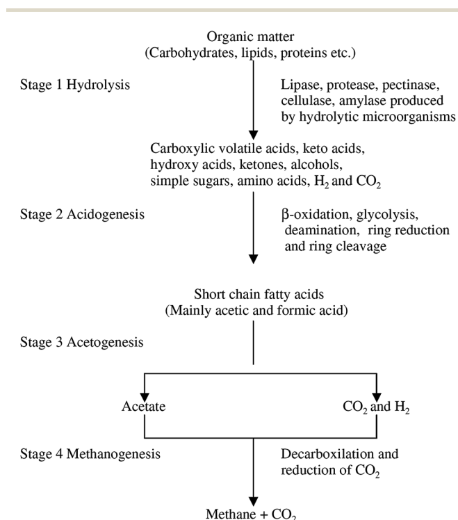
Fig. 3 Metabolic route for the conversion of organic matter to the methanogenic substrates (acetate, CO 2 and H 2 ) and finally to CH 4 and CO 2 .
