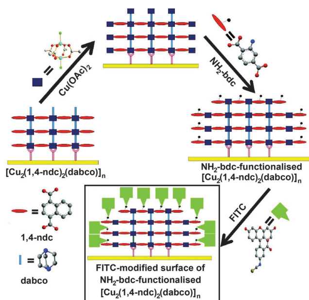
Fig. 22 Assembly of a thin film of [\text{Cu}_2(1,4\text{-ndc})_2(\text{dabco})]_n on a gold surface, followed by addition of a monolayer of 2- \text{NH}_2 -1,4- bdc on the outer surface of the film, using a layer-by-layer deposition approach. The outer layer can then be further functionalised by post-synthetic modification, in this case, tagging FITC units to the reactive amino functions. Reprinted (adapted) with permission from ref. 75. Copyright (2011) American Chemical Society.
