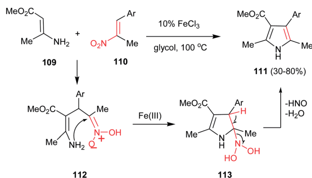
Scheme 37 FeCl 3 -catalyzed synthesis of functionalized pyrroles from enamines and nitroalkenes.
