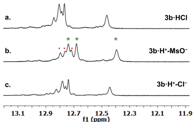
Fig. 4 ^1\text{H} NMR spectra in \text{CDCl}_3 for the pyrrolic \text{NH} region of: (a) 3b ·HCl; (b) after addition of 6 eq. of MsOH to sample a, two sets of \text{NH} signals were observed for each \alpha (·) and \beta (*) conformer; (c) after addition of 1 eq. of tetrabutylammonium chloride (TBACl) to sample b.
