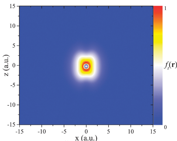
Fig. 5 The LMF f_i(\mathbf{r}) = \frac{1 - \frac{\tau_W(\mathbf{r})}{\tau(\mathbf{r})} \cdot \frac{1}{1+c^2(\mathbf{r})}} , evaluated with c = 0.5 , on the numerical grid for the C atom.
