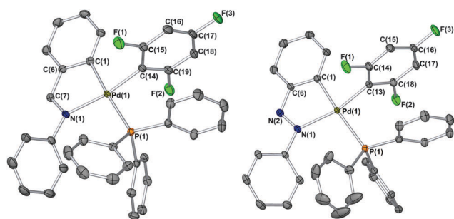
Fig. 1 X-ray structures of [Pd(phbz)(2,4,6- F_3C_6H_2 )(PPh 3 )] (left) and [Pd(phazb)-(2,4,6- F_3C_6H_2 )(PPh 3 )] (right). Selected bond angles (°) and lengths (Å): C(1)–Pd(1)–C(14) 88.49(6); C(1)–Pd(1)–N(1) 80.40(5); C(1)–Pd(1)–P(1) 175.05(4); C(14)–Pd(1)–N(1) 168.86(5); C(14)–Pd(1)–P(1) 88.55(4); N(1)–Pd(1)–P(1) 102.58(3); Pd(1)–C(1) 2.0377(14); Pd(1)–C(14) 1.9945(13); Pd(1)–N(1) 2.1534(11) and Pd(1)–P(1) 2.3756(4) for [Pd(phbz)(2,4,6- F_3C_6H_2 )-(PPh 3 )]. C(1)–Pd(1)–C(13) 89.38(8); C(1)–Pd(1)–N(1) 78.02(8); C(1)–Pd(1)–P(1) 170.65(6); C(13)–Pd(1)–N(1) 165.92(8); C(13)–Pd(1)–P(1) 88.78(6); N(1)–Pd(1)–P(1) 104.66(5); Pd(1)–C(1) 2.020(2); Pd(1)–C(13) 2.005(2); Pd(1)–N(1) 2.1427(17) and Pd(1)–P(1) 2.3746(6) for [Pd(phazb)(2,4,6- F_3C_6H_2 )(PPh 3 )].
