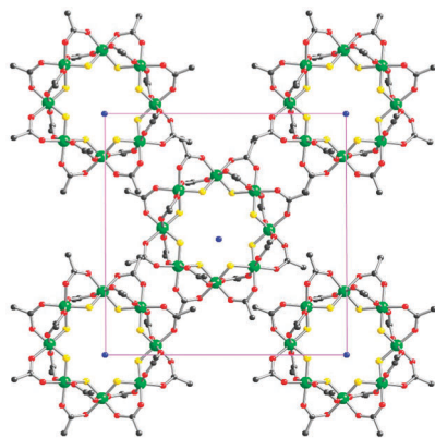
Fig. 1 Unit cell of \text{Cr}_7\text{Zn}@Ga_7\text{Zn} viewed down the crystal c axis: Ga/Cr/Zn (green), F (yellow), O (red), N (blue), C (black), Me groups omitted for clarity. See Fig. S1 (ESI†) for full molecule.
