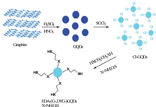
Scheme 1 A schematic route of the synthesis of functionalized GQDs with selected diamines, glycols and dithioglycols.
