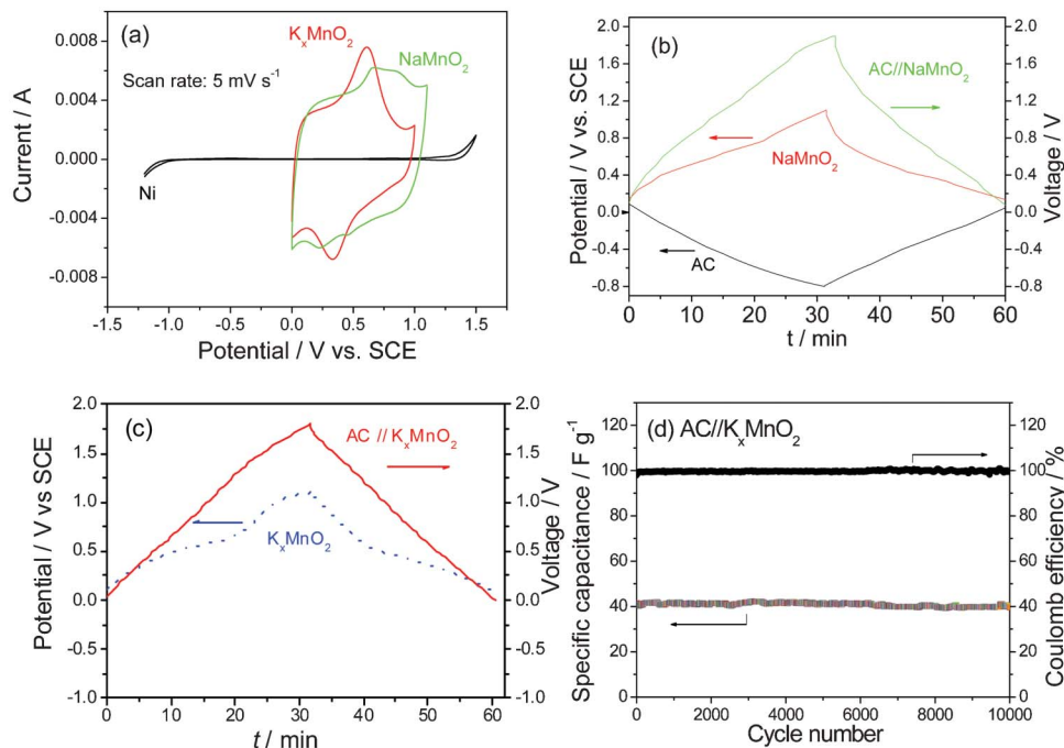
Fig. 19 (a) CV curves of \text{NaMnO}_2 and \text{K}_x\text{MnO}_2 in 0.5 mol \text{l}^{-1} \text{Na}_2\text{SO}_4 and \text{K}_2\text{SO}_4 aqueous solution, charge and discharge curves of (b) AC//AC, \text{NaMnO}_2 and AC// \text{NaMnO}_2 hybrid supercapacitors in 0.5 mol \text{l}^{-1} \text{Na}_2\text{SO}_4 aqueous solution, (c) \text{K}_x\text{MnO}_2 and AC// \text{K}_x\text{MnO}_2 hybrid supercapacitors in 0.5 mol \text{l}^{-1} \text{K}_2\text{SO}_4 aqueous solution, and (d) cycling behavior of the AC// \text{K}_x\text{MnO}_2 ASC (modified from ref. 10c and 10d).
