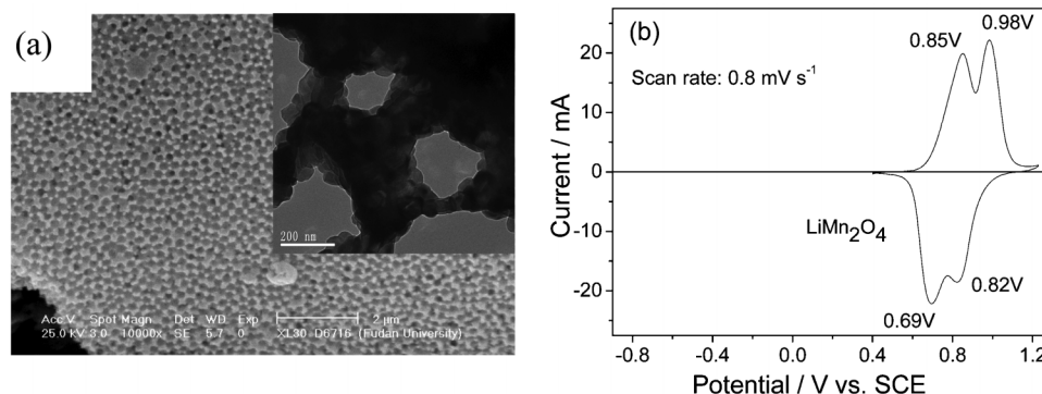
Fig. 17 (a) SEM micrograph of the porous LiMn 2 O 4 and (b) CV curve of the micrometer LiMn 2 O 4 in the saturated Li 2 SO 4 solution (modified from ref. 10b and 104).
