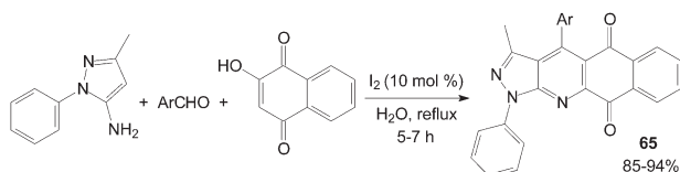
Scheme 27 Synthesis of benzo[h]pyrazolo[3,4-b]quinolines from aromatic aldehydes.
