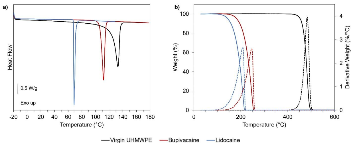
Fig. 3. Thermal and thermogravimetric behavior of UHMWPE and selected analgesic drugs. a) DSC first heating scan and b) TGA heating ramp (10 °C/min) for virgin UHMWPE (black line), bupivacaine (red line) and lidocaine (blue line). Dashed lines in b) refer to the derivative weight curves.
