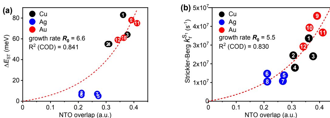
Figure 6. Relationship between {}^1\text{ICT} NTO overlap value versus (a) \Delta E_{\text{ST}} and (b) radiative decay rate of the {}^1\text{ICT} state according to the Strickler-Berg equation; fits to the data are obtained from on the twelve complexes in this work using the exponential growth function: y = A(e^{R_0 x} - 1) .
