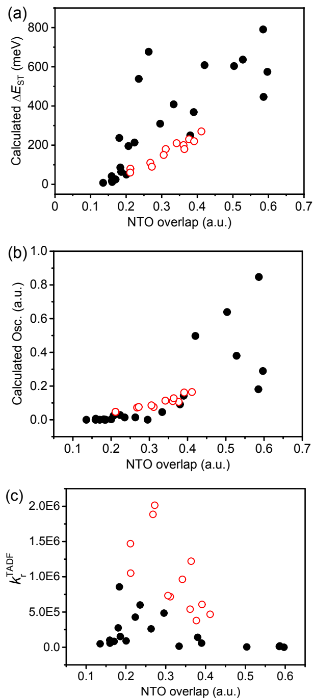
Figure 8. Relationship between NTO overlap versus (a) theoretical calculated \Delta E_{ST} , (b) calculated S_1 state oscillator strength and (c) TADF radiative decay rate in organic TADF molecules, data of organometallic TADF complexes newly reported in this paper are shown as empty red circles.
