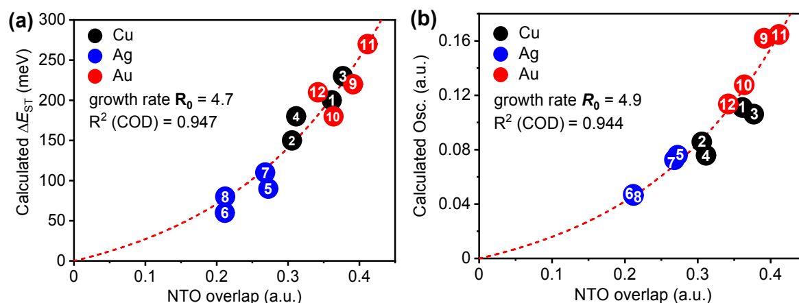
Figure 5. Relationship between {}^1\text{ICT} NTO overlap value versus theoretically calculated (a) \Delta E_{\text{ST}} and (b) oscillator strength of the S_1 state by TD-DFT method; fits to the data are obtained using the exponential growth function: y = A(e^{R_0 x} - 1) .
