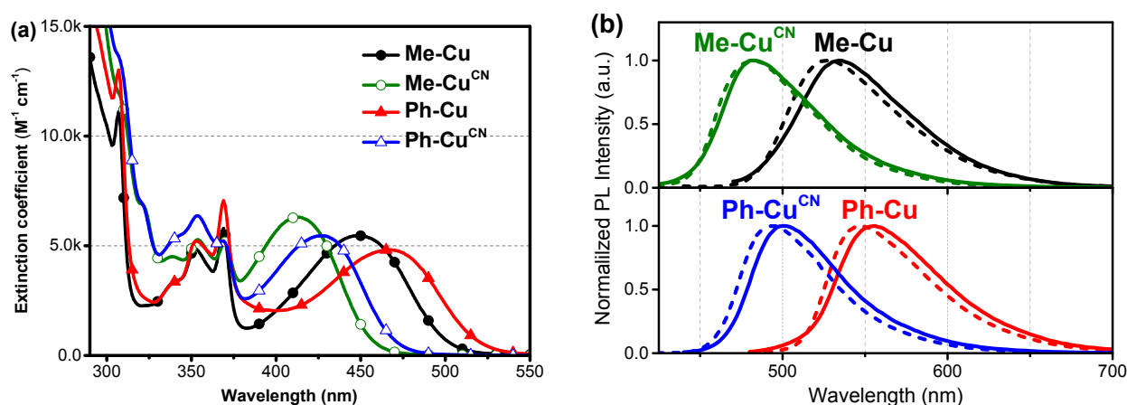
Figure 3. (a) Absorption and (b) emission spectra of Cu-based complexes. Absorption spectra recorded in toluene solution at room temperature and emission spectra in doped PS (1 wt%) films at room temperature (solid) and 77 K (dash).
