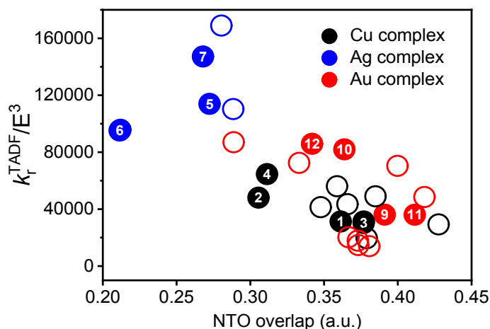
Figure 7. Relationship between the reduced TADF radiative decay rate versus NTO overlap of the ^1\text{ICT} state. The closed symbols are from this work and the open symbols are for previously reported (carbene)M(carbazolyl) complexes. See the SI for the identities of the literature complexes.
