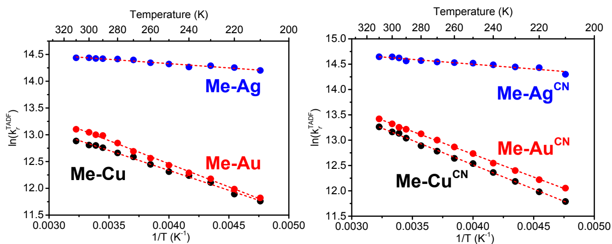
Figure 4. Fits to the temperature dependent TADF radiative decay rate from 210 to 310 K according to the full kinetic dynamic scheme.
