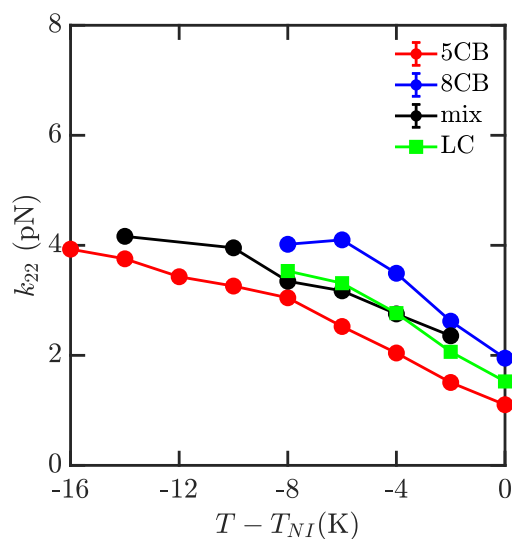
Figure 7. Predicted bulk twist elastic k_{22} constants for 5CB/8CB binary mixture. The curves are defined analogously to Figure 6.
