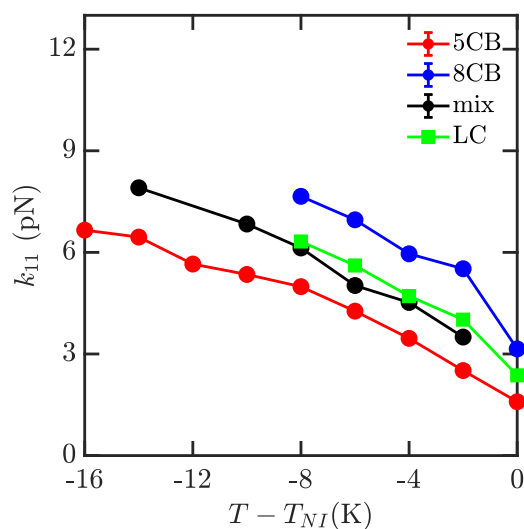
Figure 6. Bulk elastic constant k_{11} for the 5CB/8CB binary mixture ( x_{5CB} = x_{8CB} = 0.5 ) (black) compared with the calculated k_{11} constants for 5CB 8 (red) and 8CB (blue). The LC curve (green) is a linear combination of the elastic constants of 5CB and 8CB, weighted by mole fraction.
