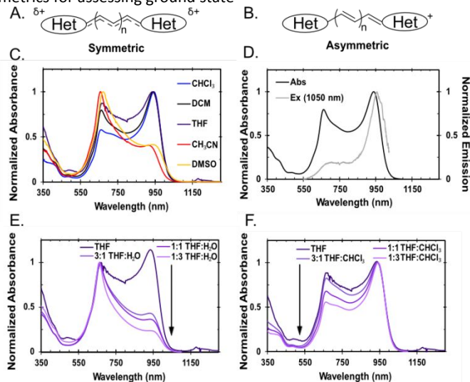
Figure 3. A/B) Schematic of symmetric state (delocalized charge, A) and asymmetric state (dipolar, charge is localized on one heterocycle, B). C) Absorbance of 10 (normalized to \lambda_{\text{max}} ) in a range of nonpolar and polar solvents. D) Normalized absorption spectra (Abs, black) and excitation spectra (Ex, grey, excitation from 515–1025 nm and collection 1050 nm) of 10 in DCM. E) Absorption spectra of 10 normalized at 663 nm in a solution of tetrahydrofuran (THF, 0.01 mM) supplemented with increasing amounts of H 2 O. F) Absorption spectra of 10 normalized at 938 nm in a solution of THF (0.01 mM) supplemented with increasing amounts of CHCl 3 .
