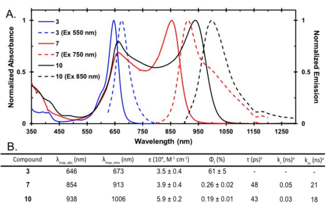
Figure 2. Photophysical data of silicon fluorophores. A) Normalized absorbance (solid) and emission (dotted) in dichloromethane (DCM). B) Photophysical characterization of 3 , 7 , 10 in DCM. a Error and experimental in detail in Figure S8.
