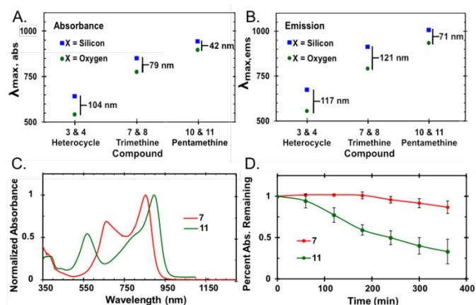
Figure 5. Comparison of silicon and oxygen xanthenes polymethines. A/B) \lambda_{\max} of silicon- (blue square) and oxygen- (green circle) containing polymethine fluorophores in DCM. The values depicted on the plot indicate the degree of red-shift imparted by silicon. A) Absorbance. B) Emission. C) Normalized absorbance spectra of 7 and 11 in DCM. D) Percent absorbance remaining at \lambda_{\max,abs} of 7 and 11 with continuous irradiation at 730 nm ( 146 \text{ mW/cm}^2 ) over 6 hours. Error is the standard deviation of three experiments.
