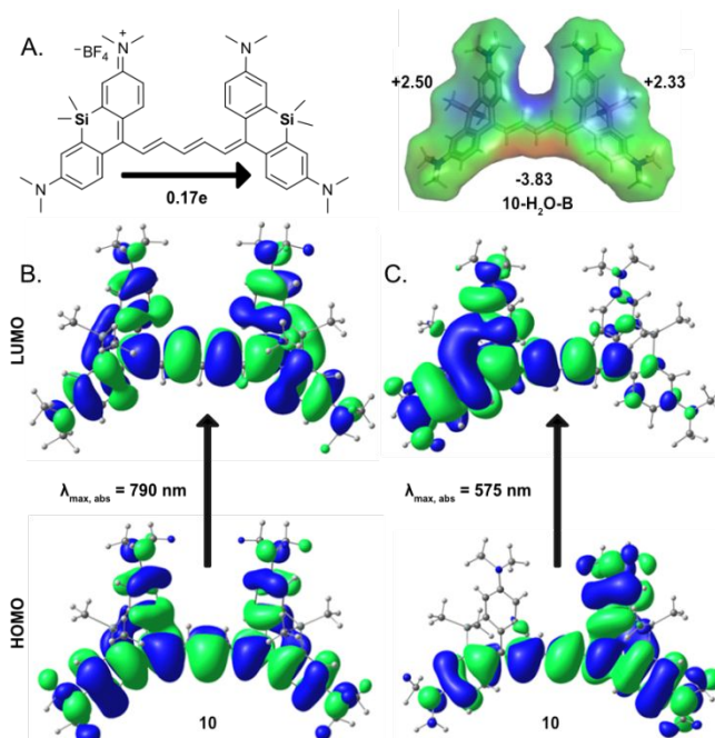
Figure 4. A) Conformer 10-H 2 O-B shows desymmetrization of 0.17e charge transfer toward the right heterocycle represented schematically and by electron density map. B) Frontier molecular orbitals of Wigner sampled structures of 10 computed with CIS(D)/cc-pvdz-RI correspond to \lambda_{\max, \text{abs}} of 790 nm, show complete electron delocalization. C) HOMO and LUMO of sampled structures of 10 with predicted \lambda_{\max, \text{abs}} of 575 nm show asymmetric character in their electronic structure.
