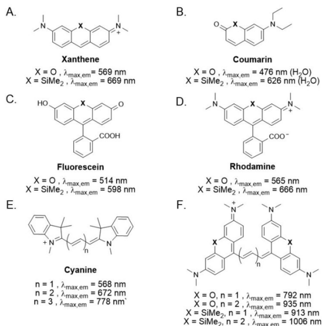
Figure 1. Fluorophore scaffolds. A) Xanthenes scaffold, the first fluorophore where silicon was incorporated. 4 B) Coumarin scaffold. 11 C) Fluorescein scaffold. 10 D) Rhodamine scaffold. 10 E) Cyanine scaffold: a classic polymethine dye. 12 F) This work on silicon polymethines and their oxygen counterparts. 13
